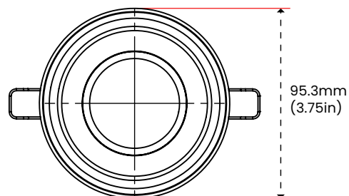
Sensor with ceiling mount and high-bay lens accessories (WMAP-CMK-HBL)
